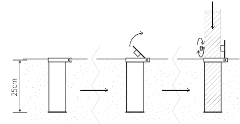
Base Empotrable
